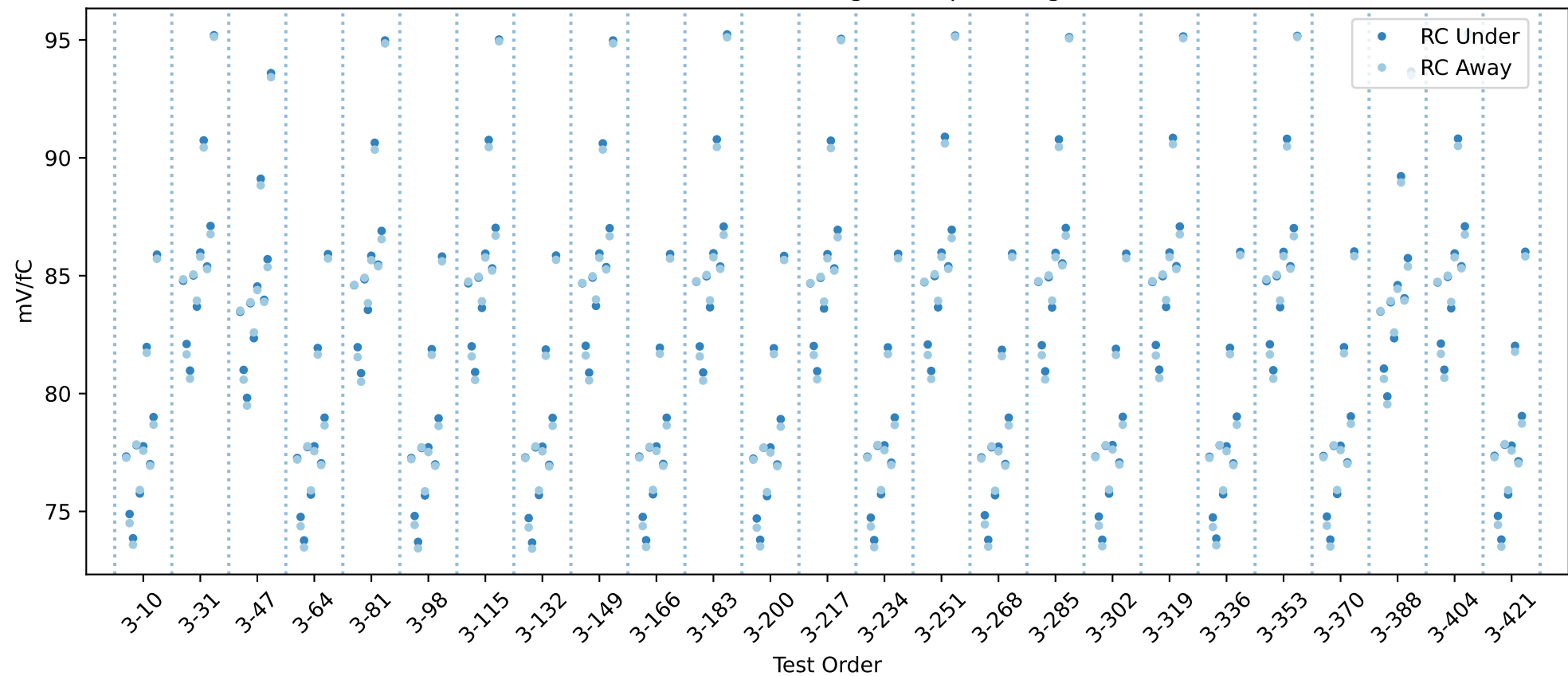
20USBHX2004653 RC gain chip averages
