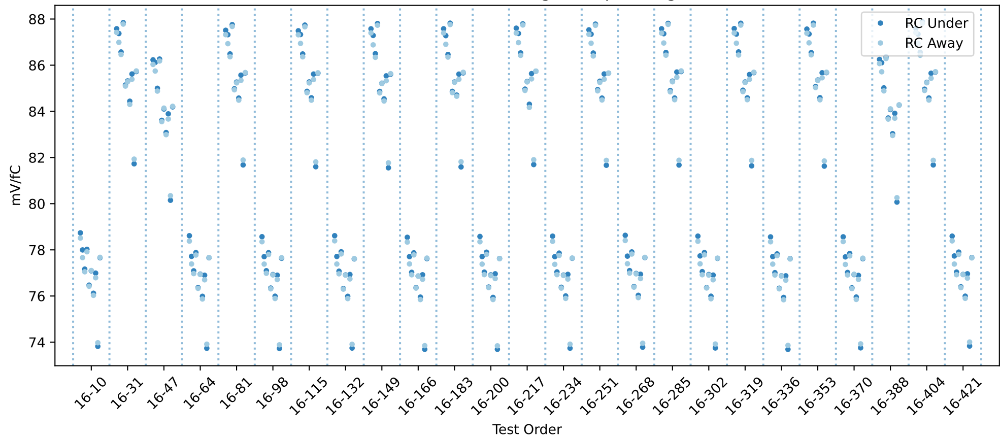
20USBHX2004562 RC gain chip averages
