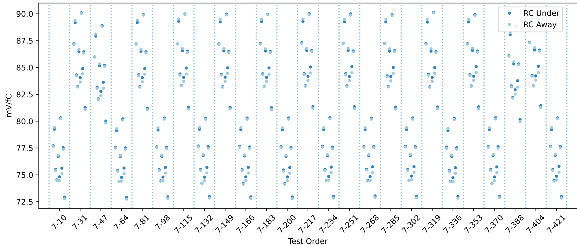
20USBHX2004564 RC gain chip averages
