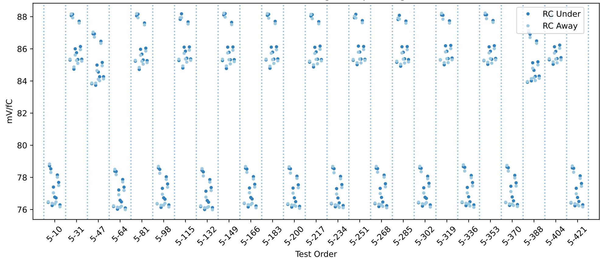
20USBHX2004652 RC gain chip averages
