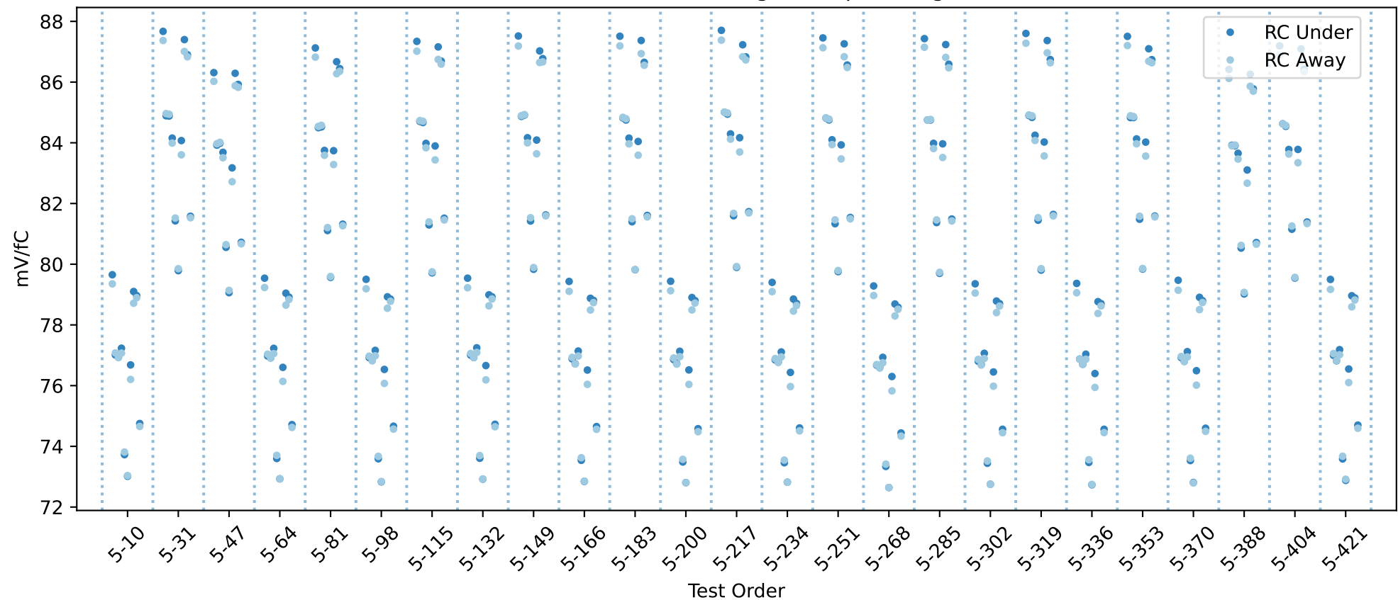
20USBHX2004830 RC gain chip averages
