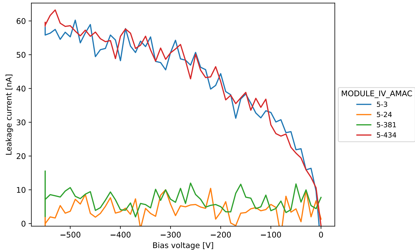
20USBML1237565 standard IV
