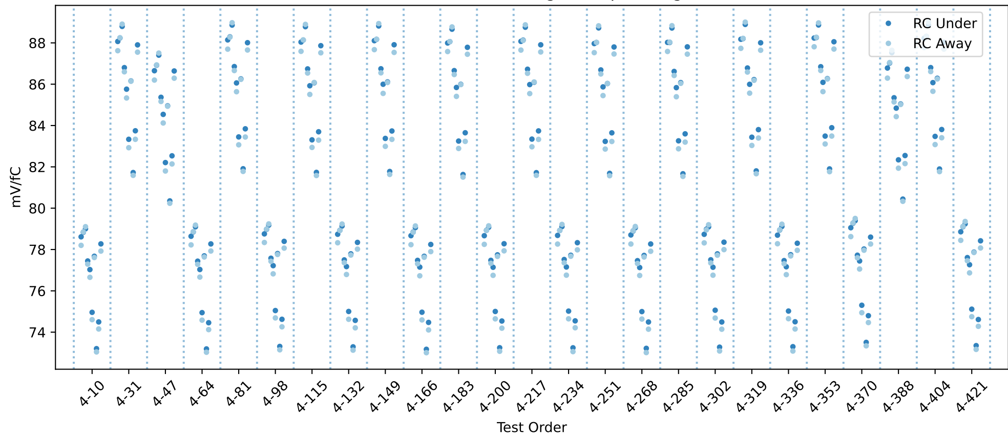
20USBHX2004835 RC gain chip averages
