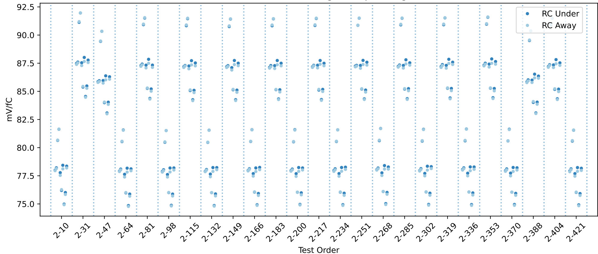
20USBHX2004878 RC gain chip averages
