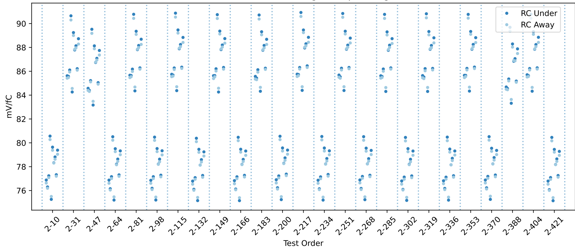
20USBHX2004879 RC gain chip averages
