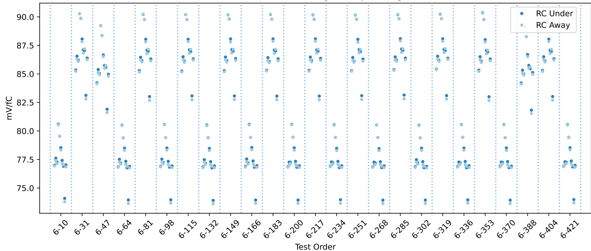
20USBHX2004892 RC gain chip averages
