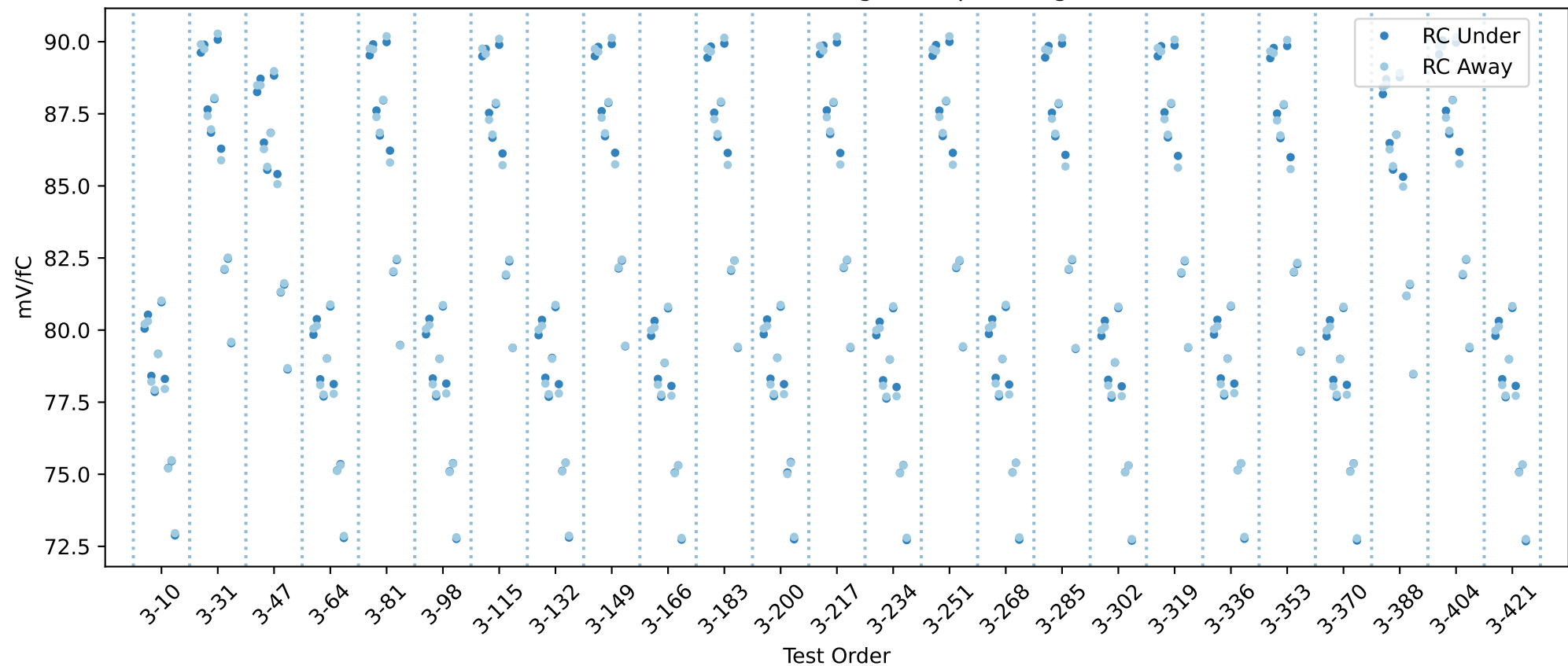
20USBHX2004837 RC gain chip averages
