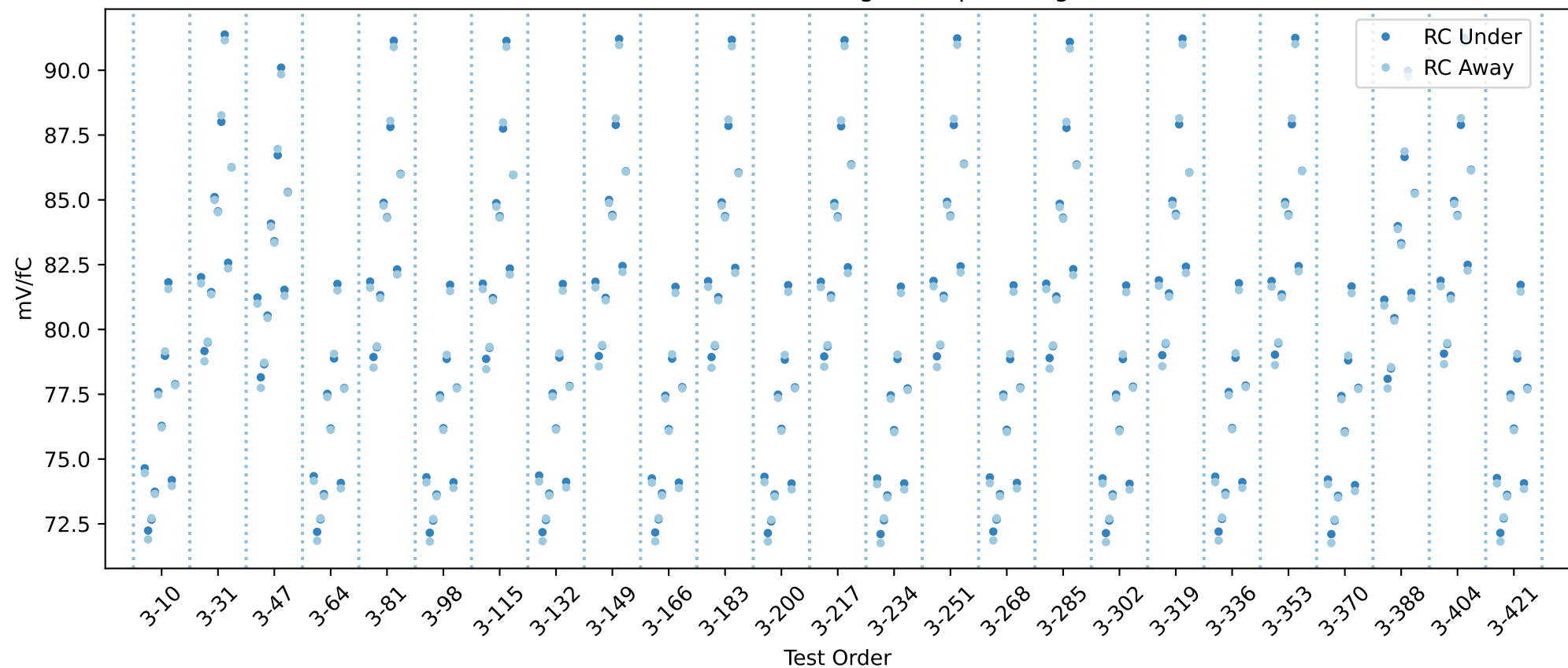
20USBHX2004840 RC gain chip averages
