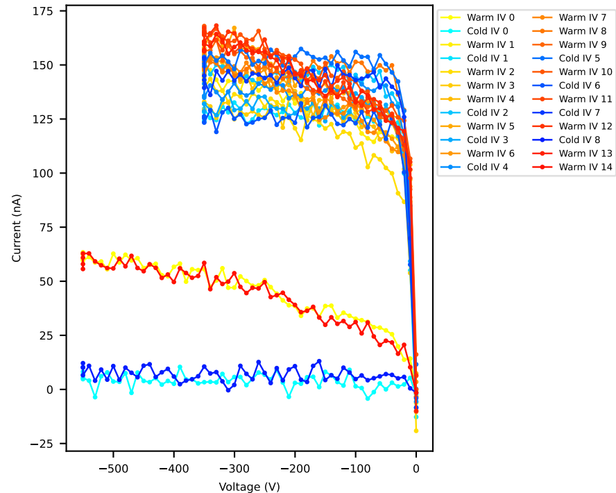
20USBML1237651 IV Results Throughout TC
