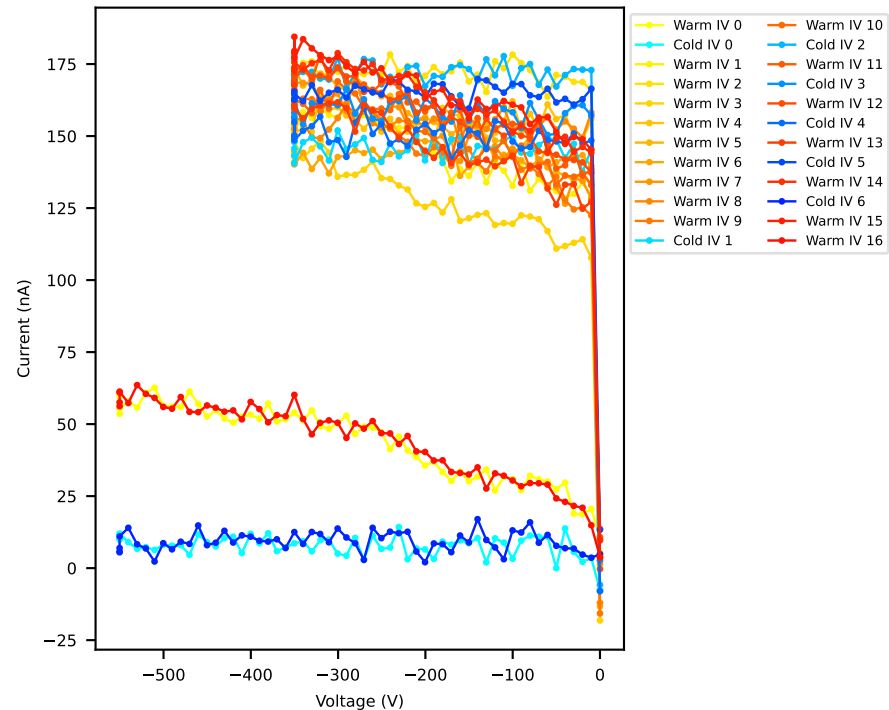
20USBML1237659 IV Results Throughout TC
