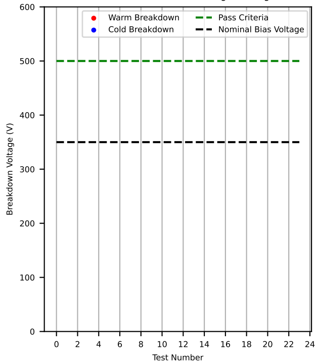
20USBML1237659 Breakdown Voltage Throughout TC
