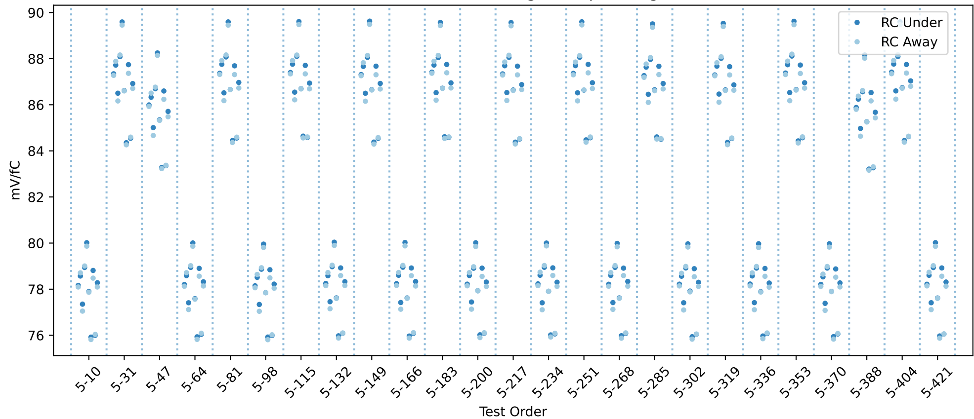
20USBHX2004898 RC gain chip averages
