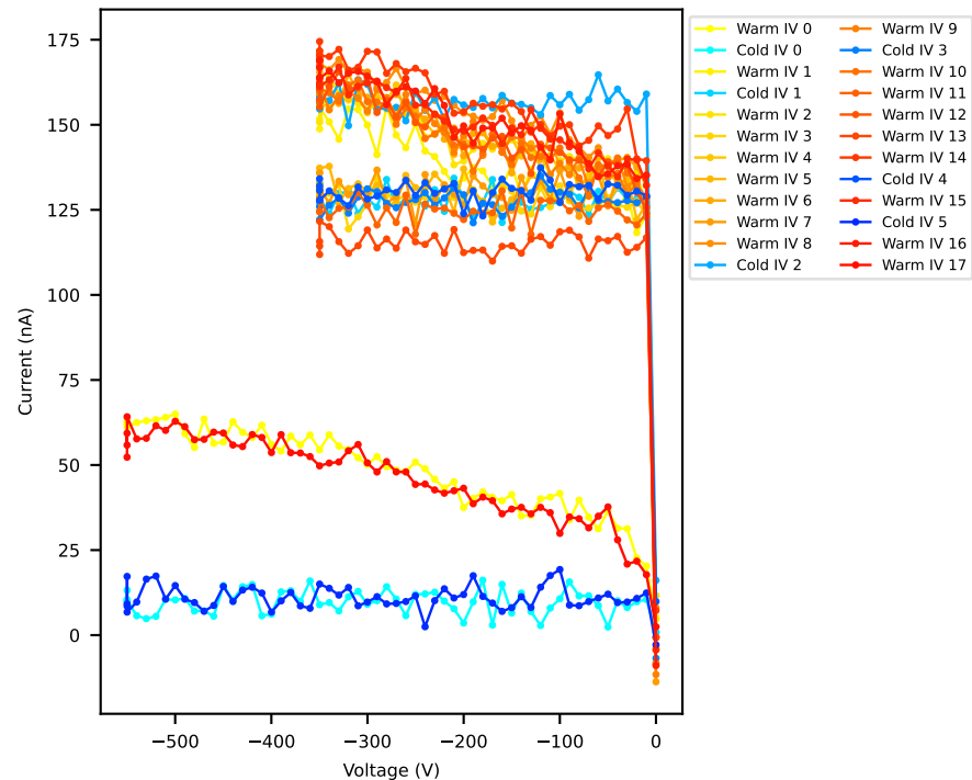
20USBML1237667 IV Results Throughout TC
