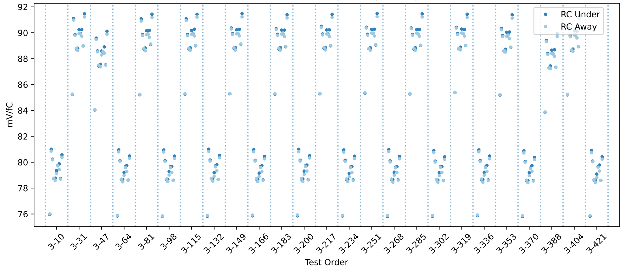
20USBHX2004882 RC gain chip averages
