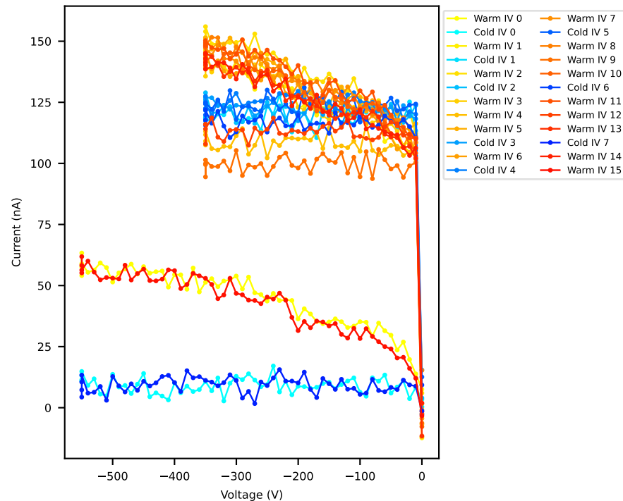
20USBML1237672 IV Results Throughout TC
