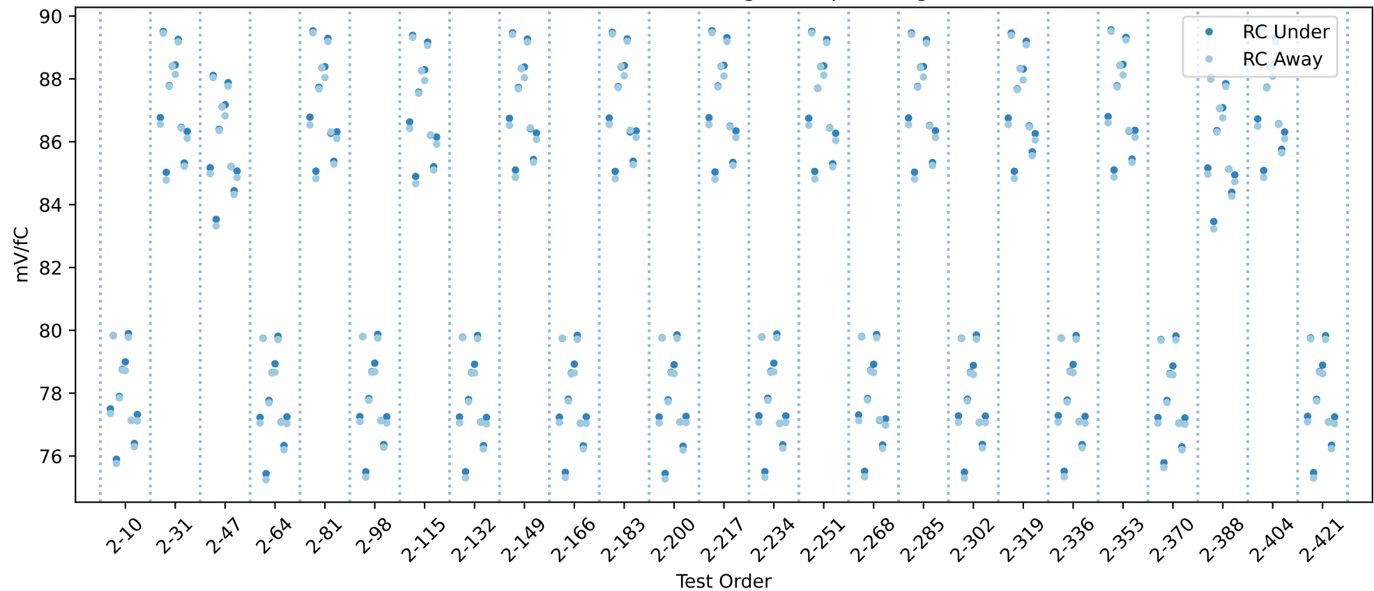
20USBHX2004900 RC gain chip averages
