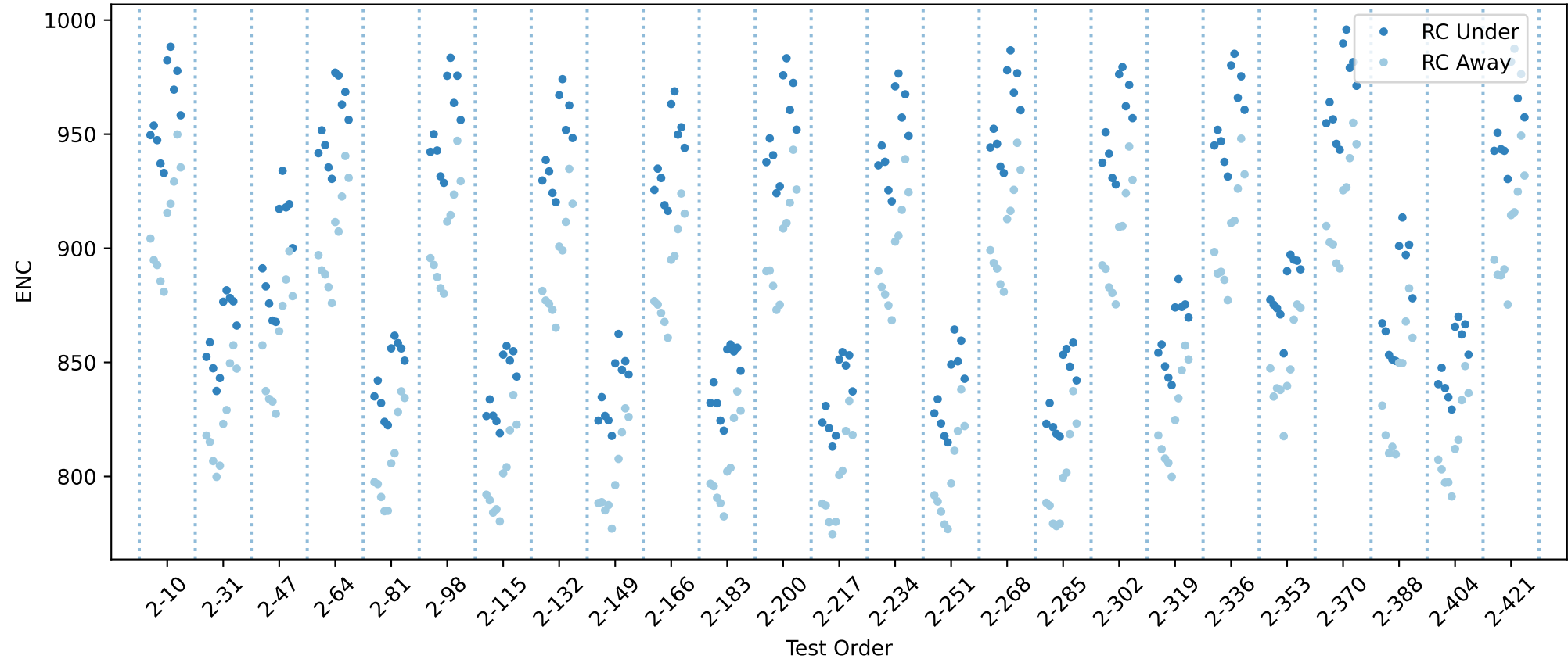
20USBHX2005064 RC innse chip averages
