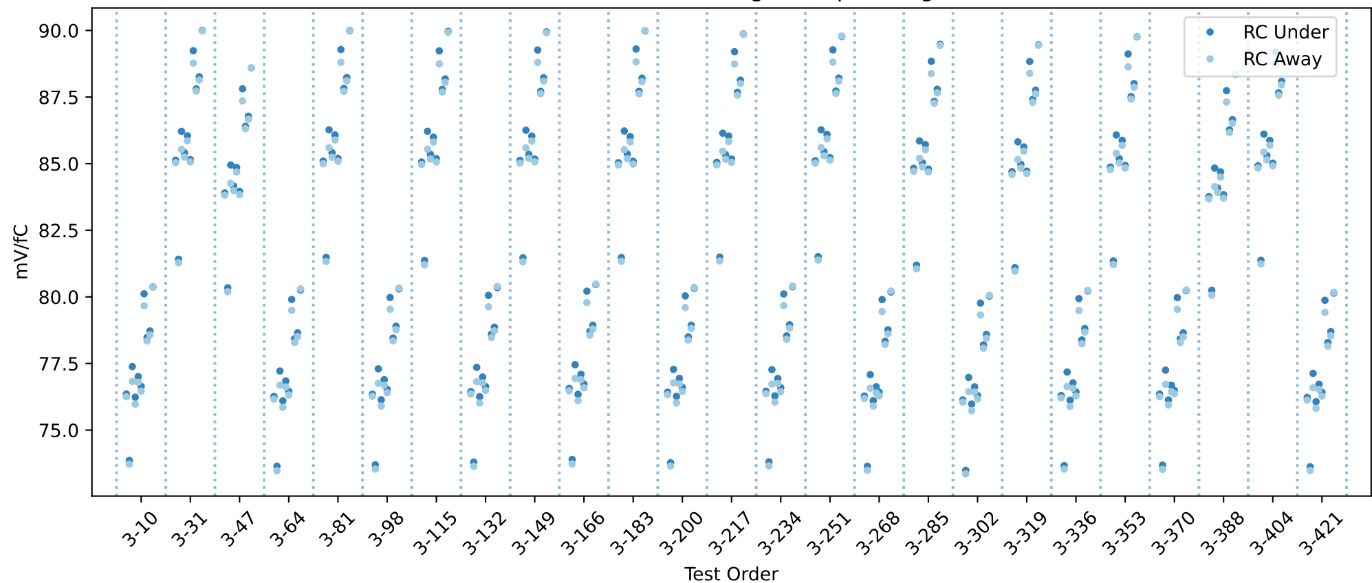
20USBHX2005079 RC gain chip averages
