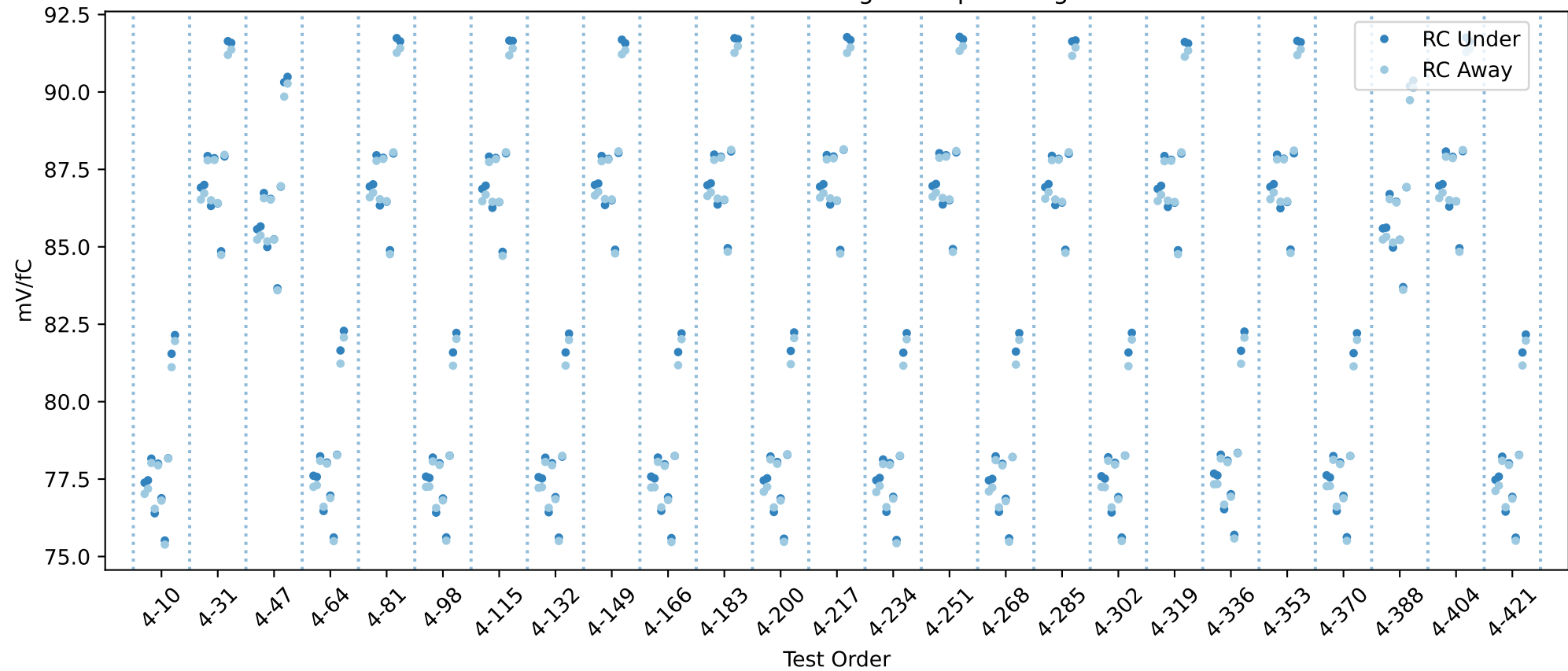
20USBHX2004982 RC gain chip averages
