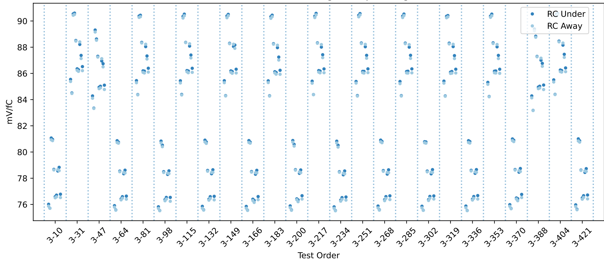
20USBHX2005049 RC gain chip averages
