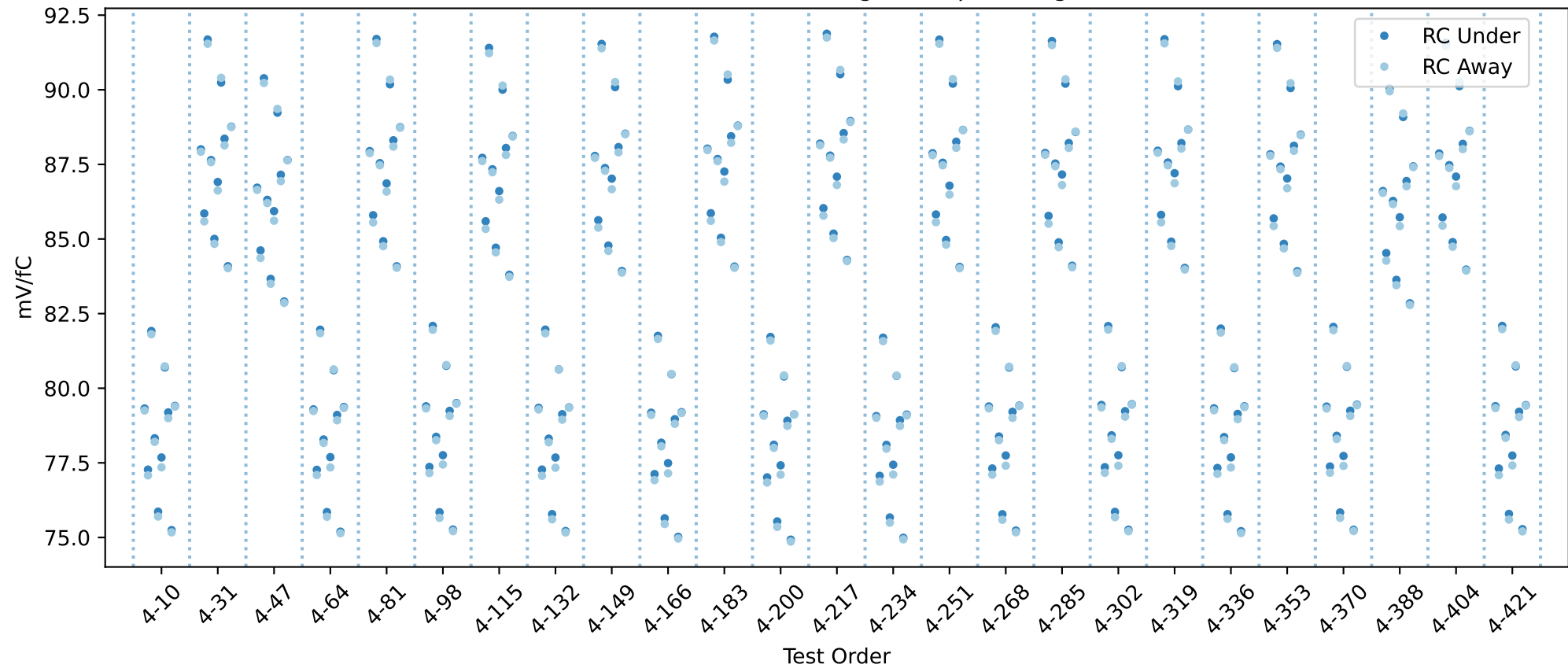
20USBHX2005044 RC gain chip averages
