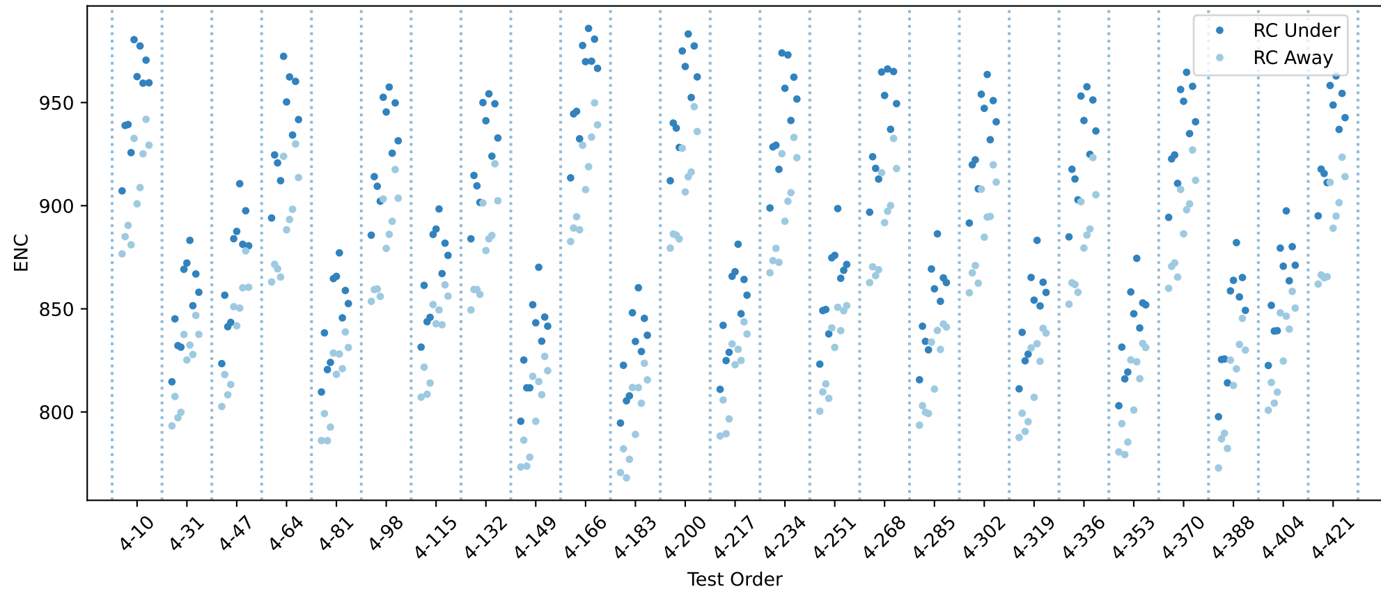
20USBHX2005044 RC innse chip averages
