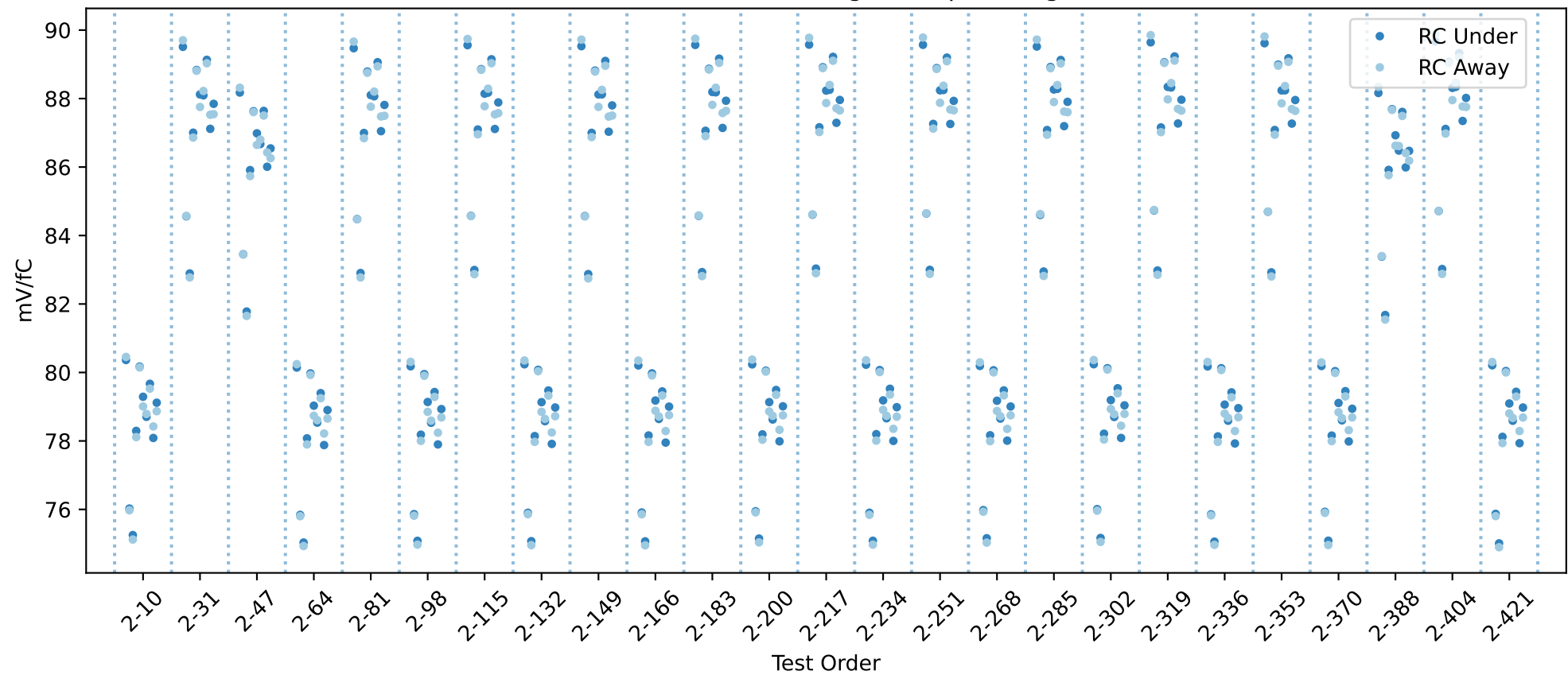
20USBHX2005054 RC gain chip averages
