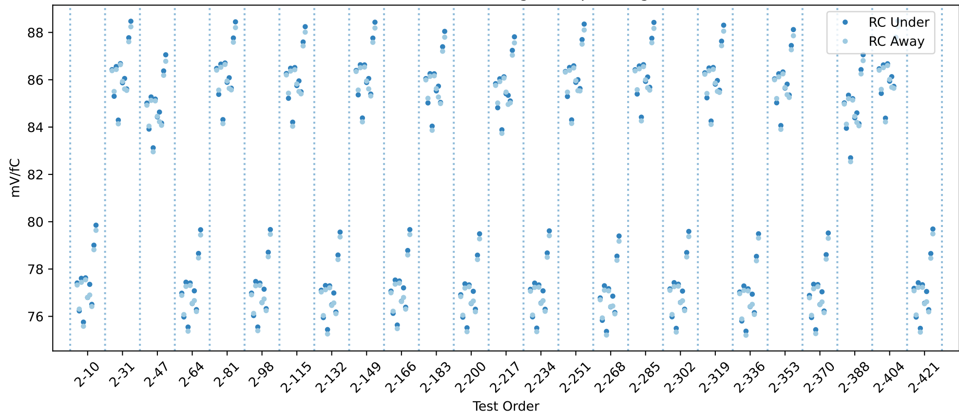
20USBHX2005055 RC gain chip averages
