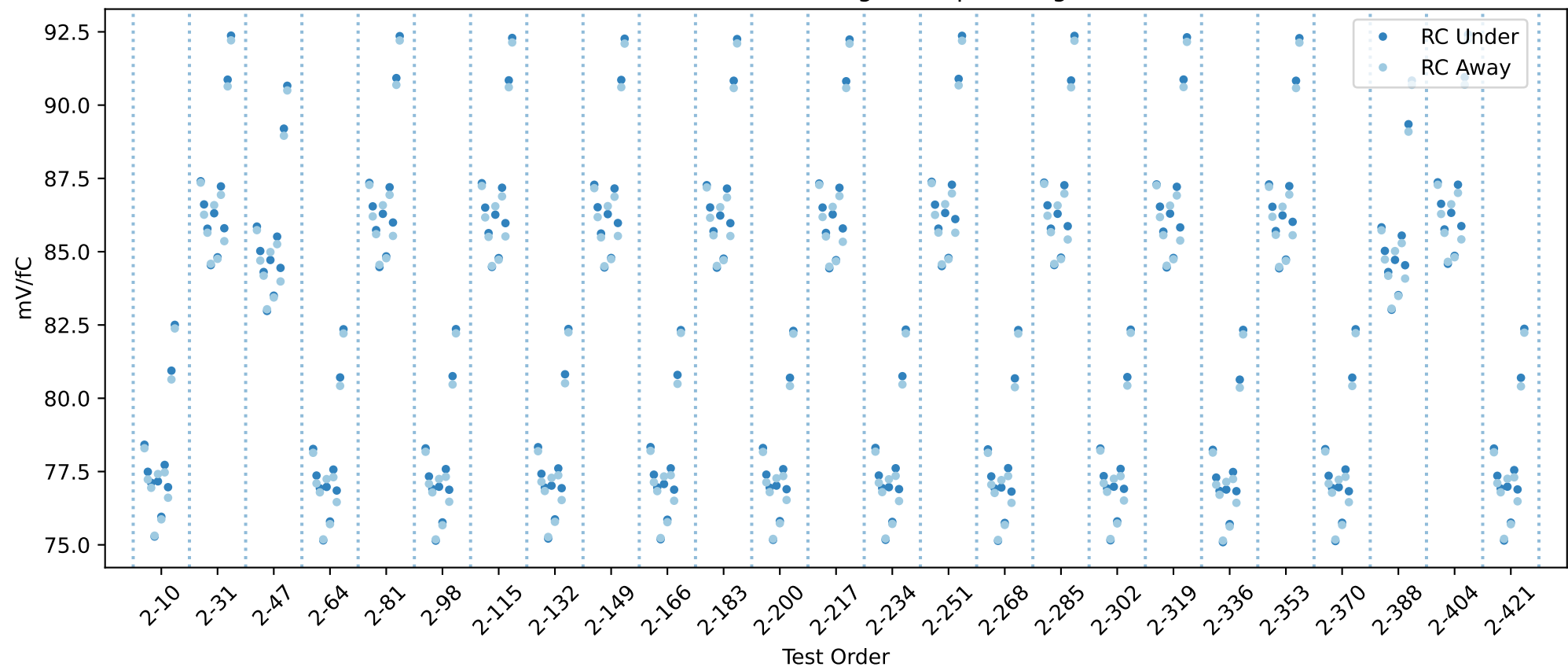
20USBHX2005056 RC gain chip averages
