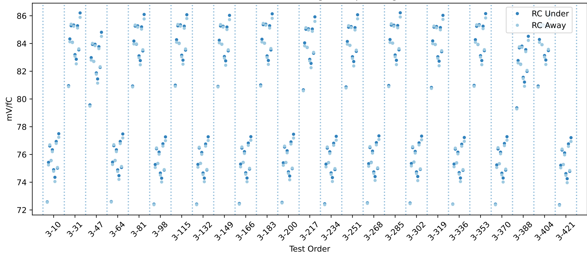
20USBHX2005083 RC gain chip averages
