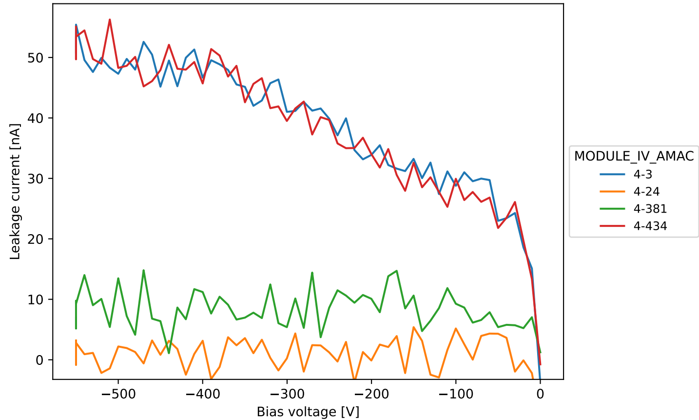
20USBML1237959 standard IV
