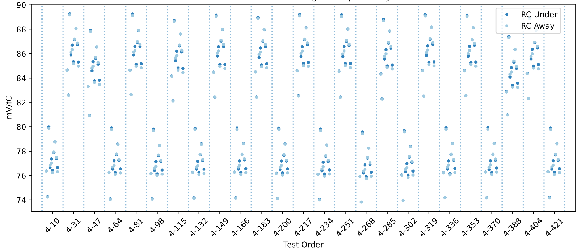
20USBHX2005004 RC gain chip averages
