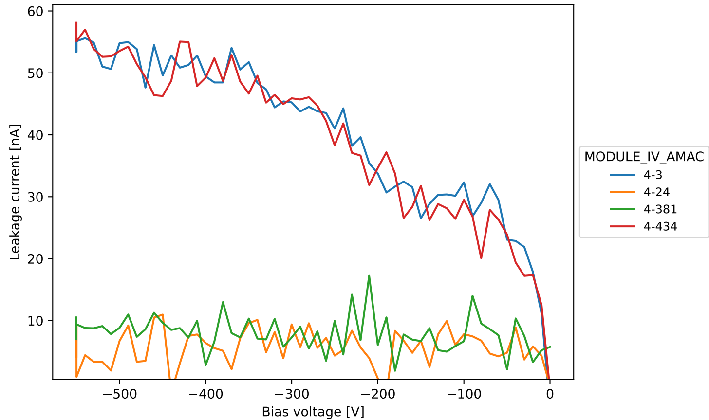
20USBML1237964 standard IV
