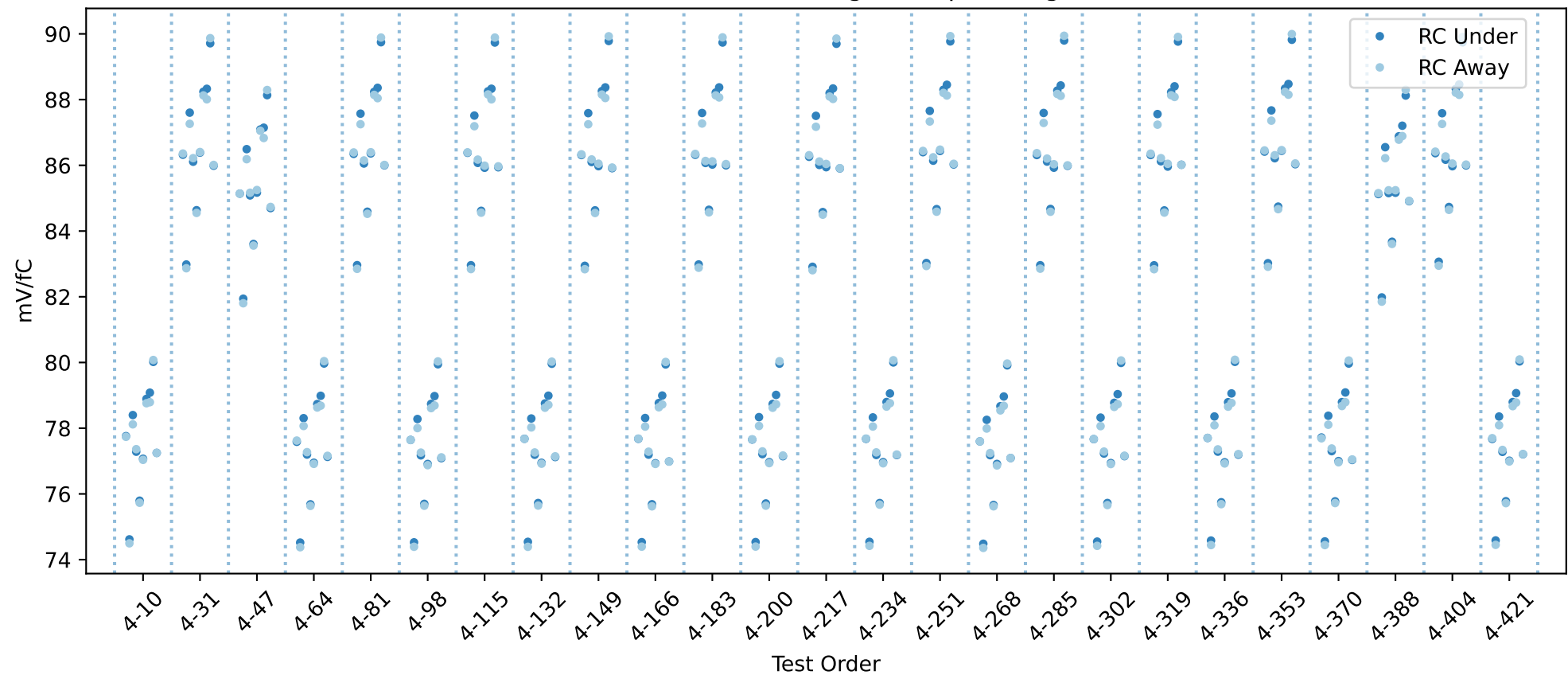
20USBX2004988 RC gain chip averages
