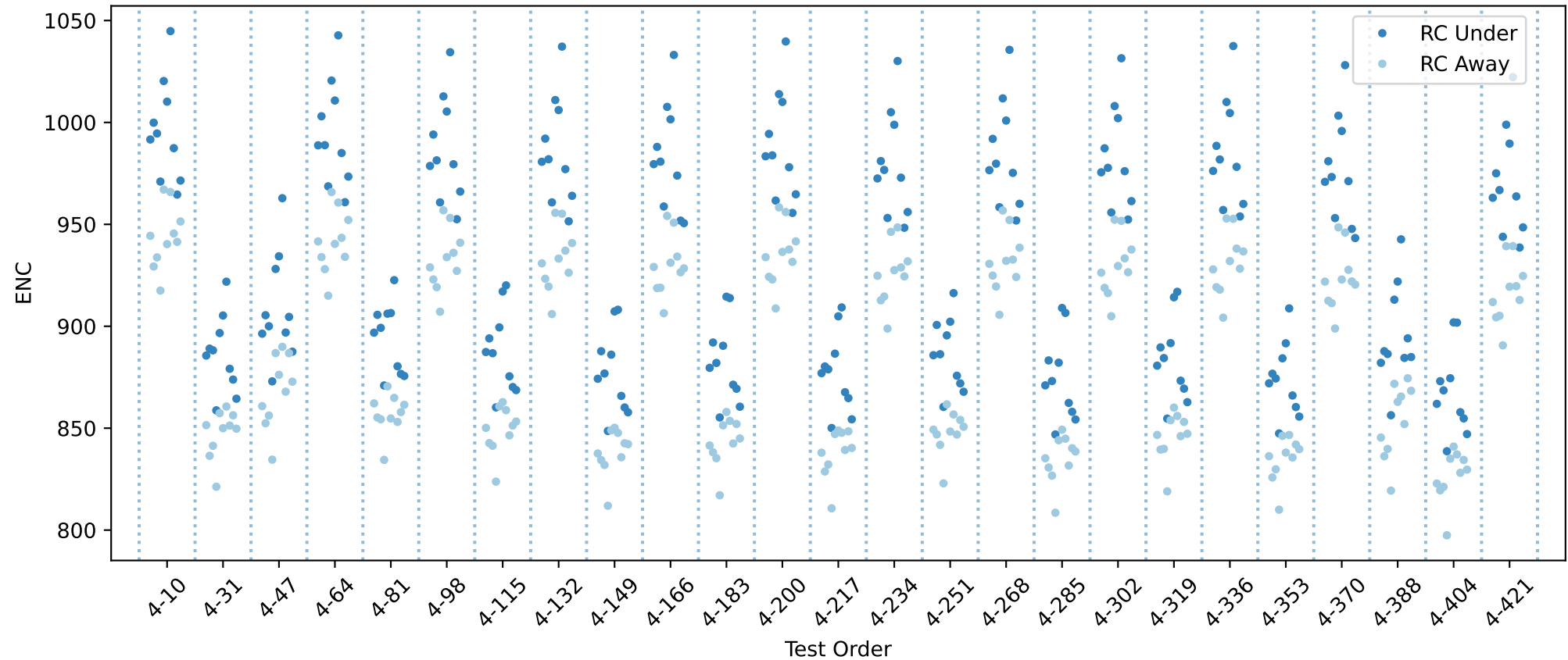
20USBHX2004988 RC innse chip averages
