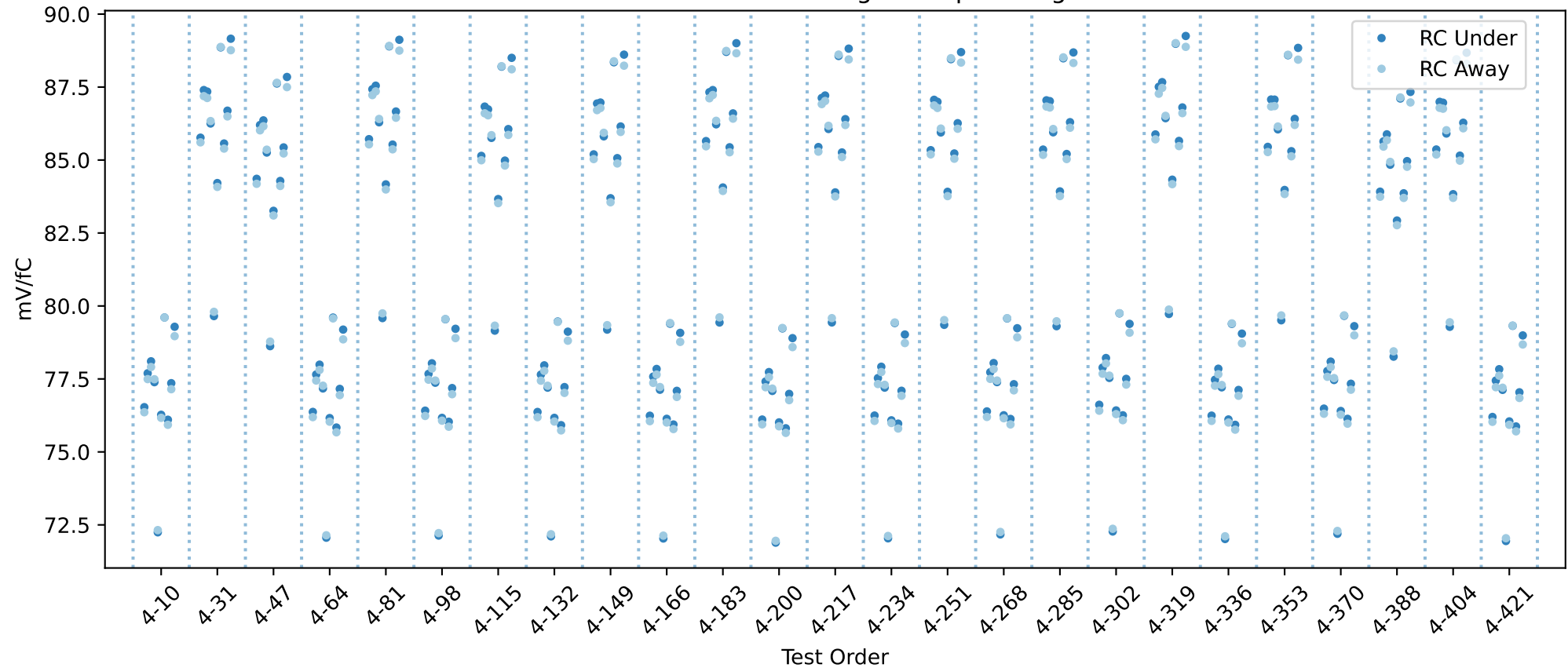
20USBHX2004989 RC gain chip averages
