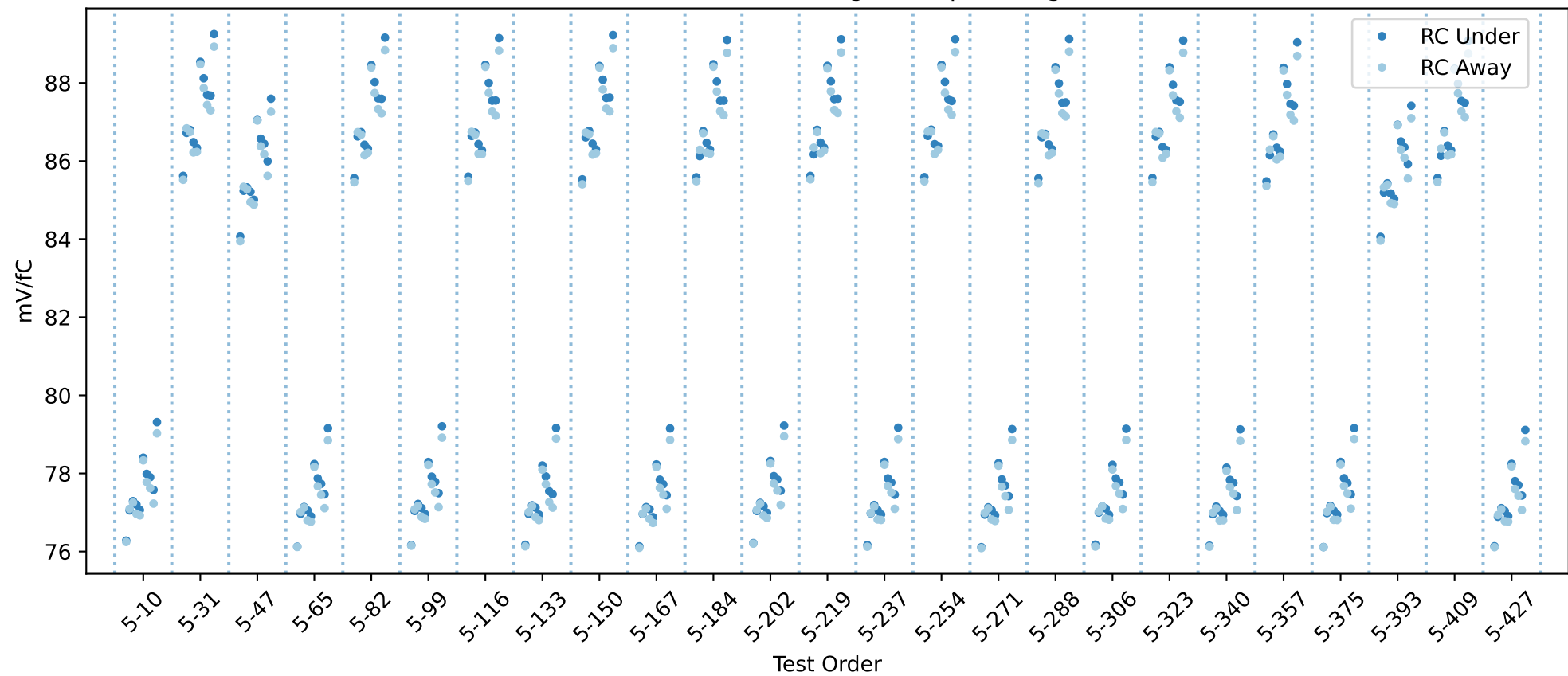
20USBHX2004981 RC gain chip averages
