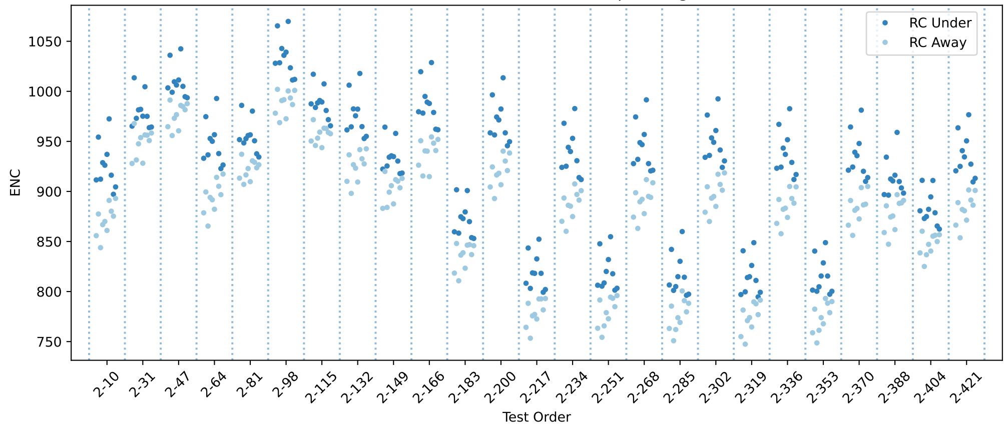
20USBHX2005034 RC innse chip averages
