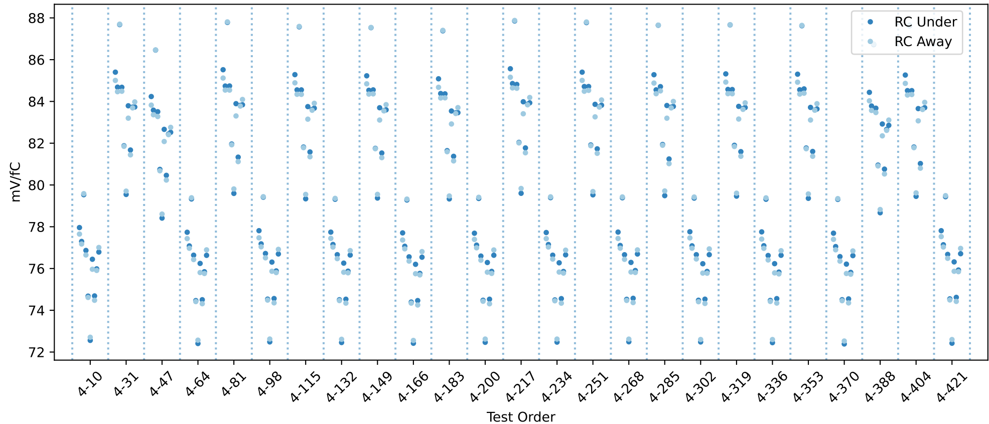
20USBHX2005035 RC gain chip averages
