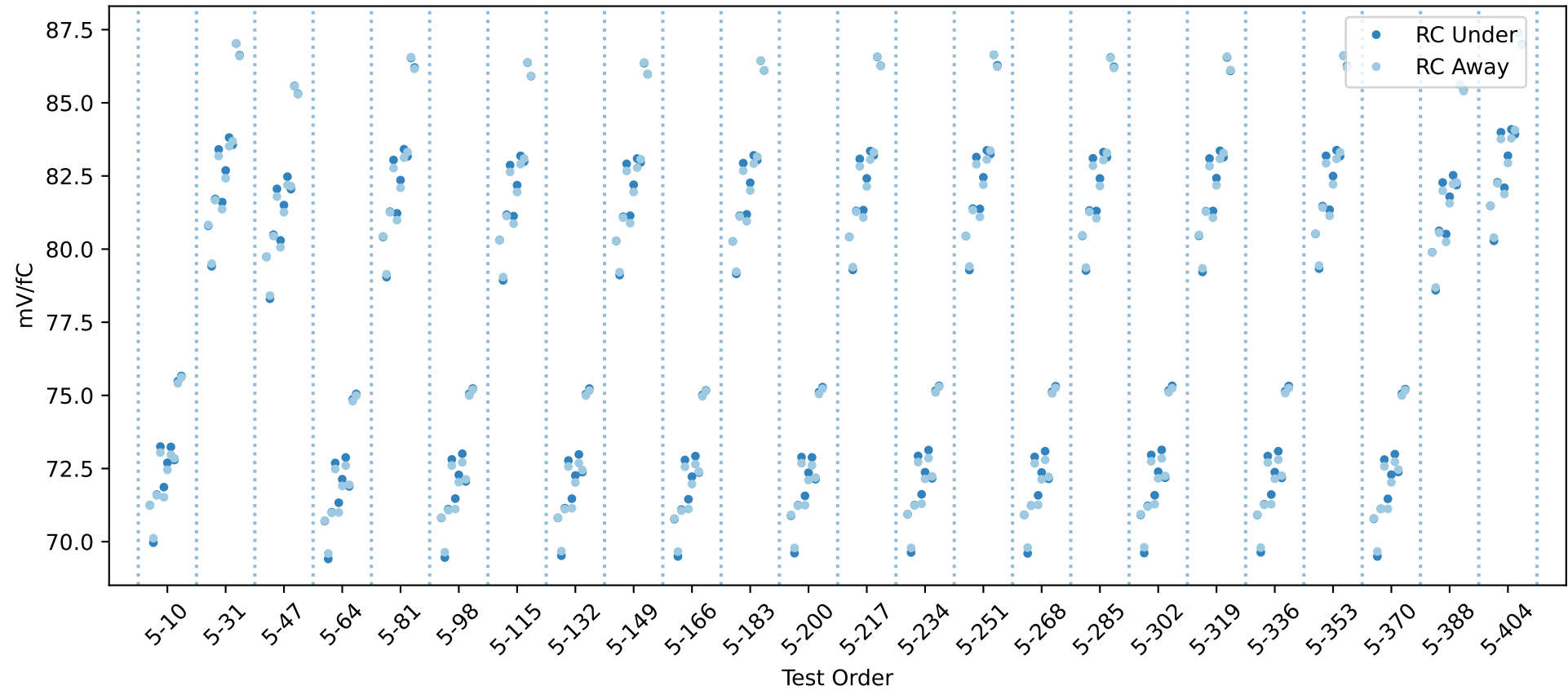
20USBHX2005065 RC gain chip averages
