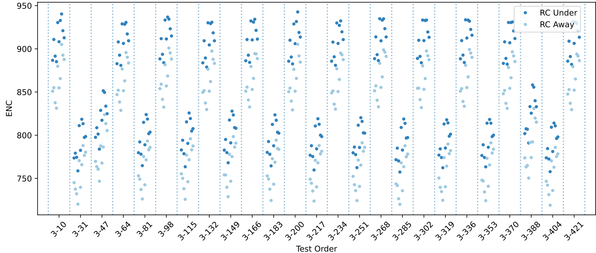
20USBHX2005292 RC innse chip averages
