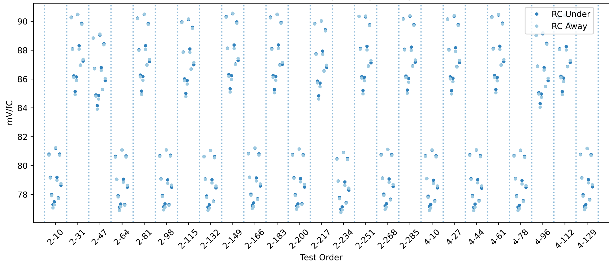
20USBHX2005074 RC gain chip averages
