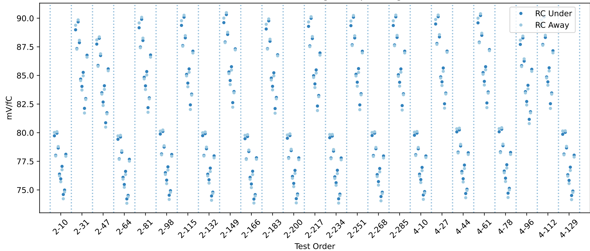
20USBHX2005295 RC gain chip averages
