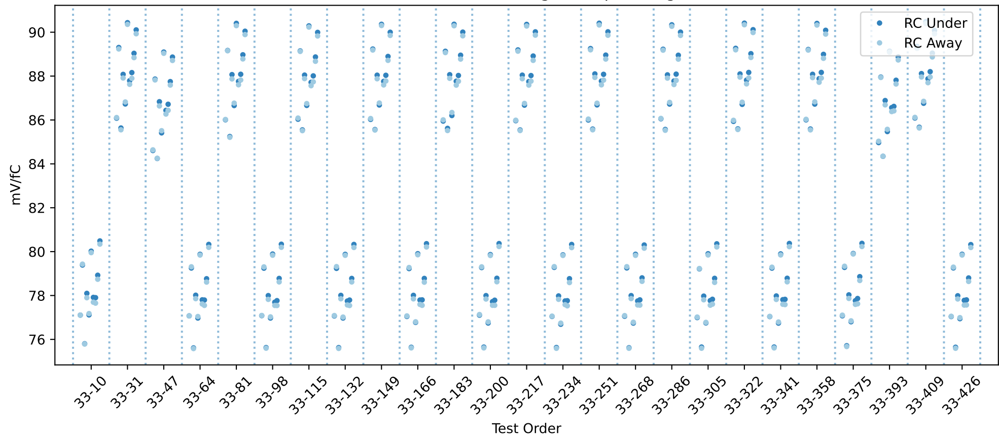
20USBHX2005069 RC gain chip averages
