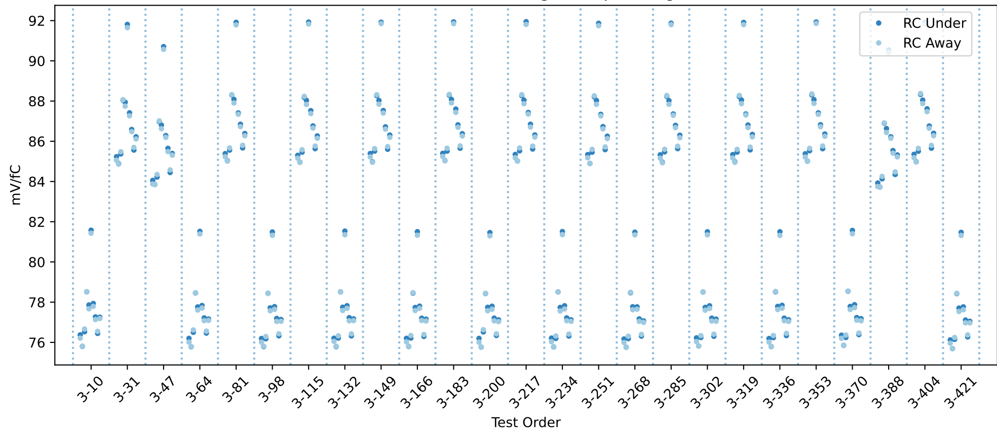
20USBX2005298 RC gain chip averages
