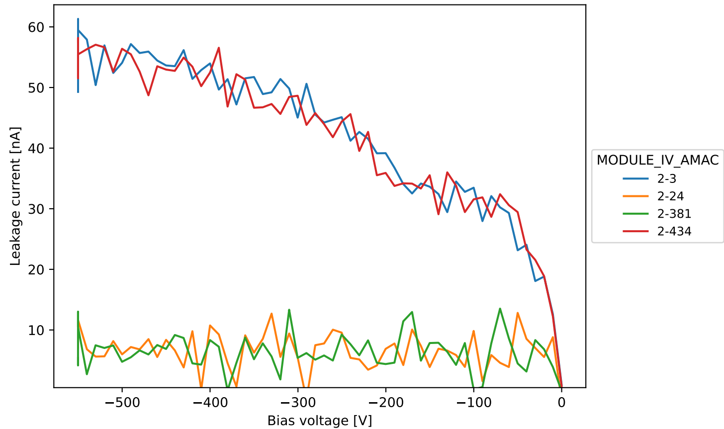
20USBML1238362 standard IV
