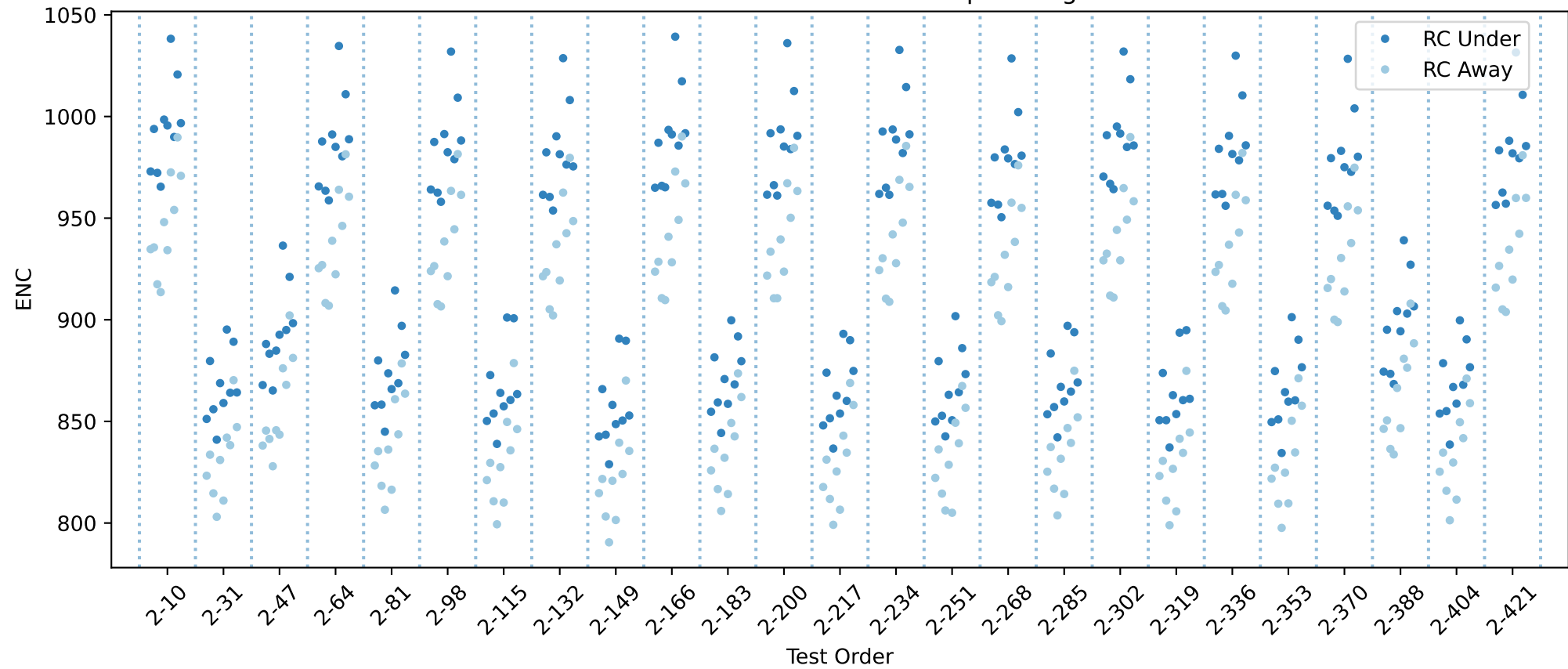
20USBHX2005221 RC innse chip averages
