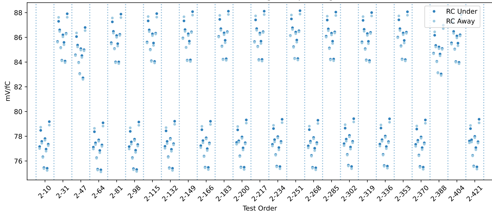
20USBHX2005249 RC gain chip averages
