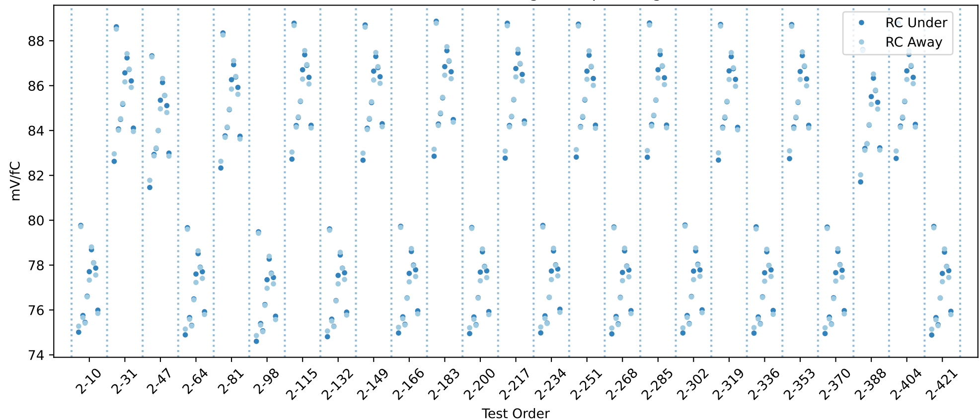
20USBHX2005253 RC gain chip averages
