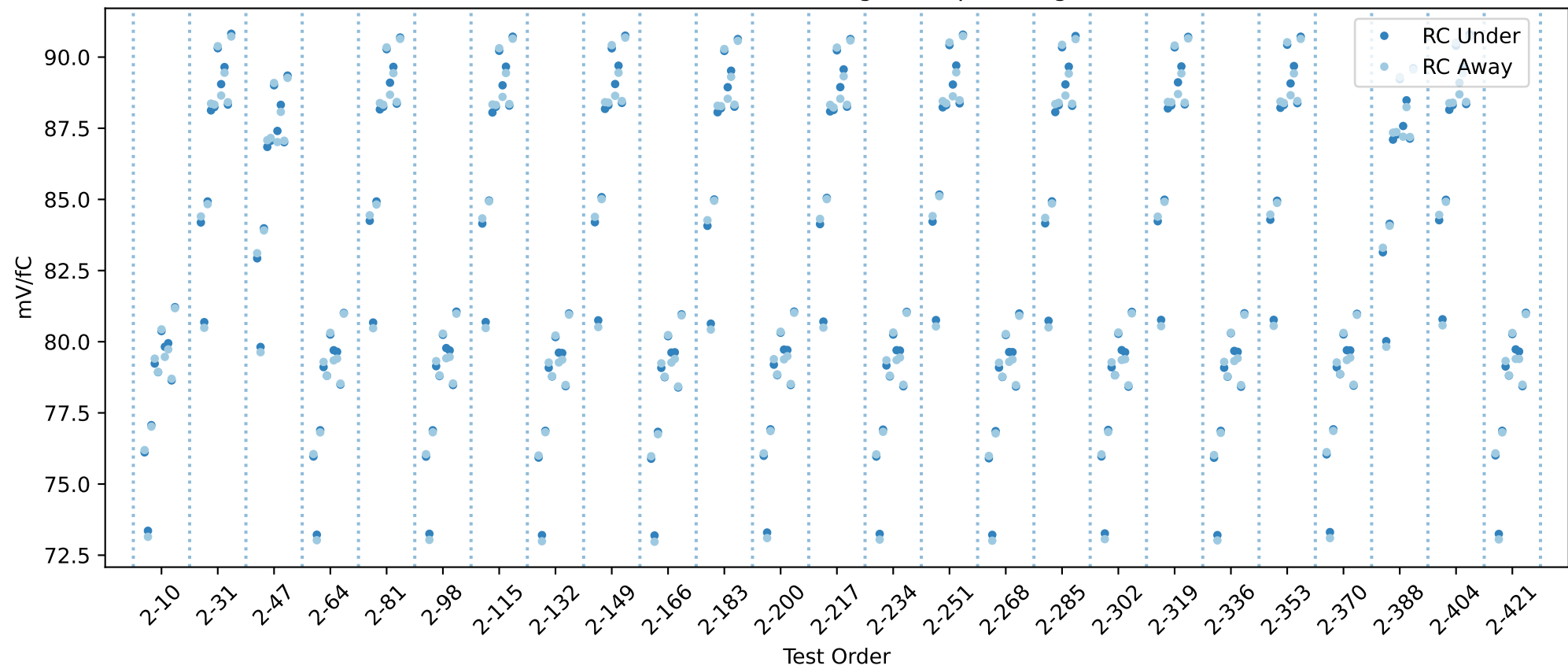
20USBHX2005225 RC gain chip averages
