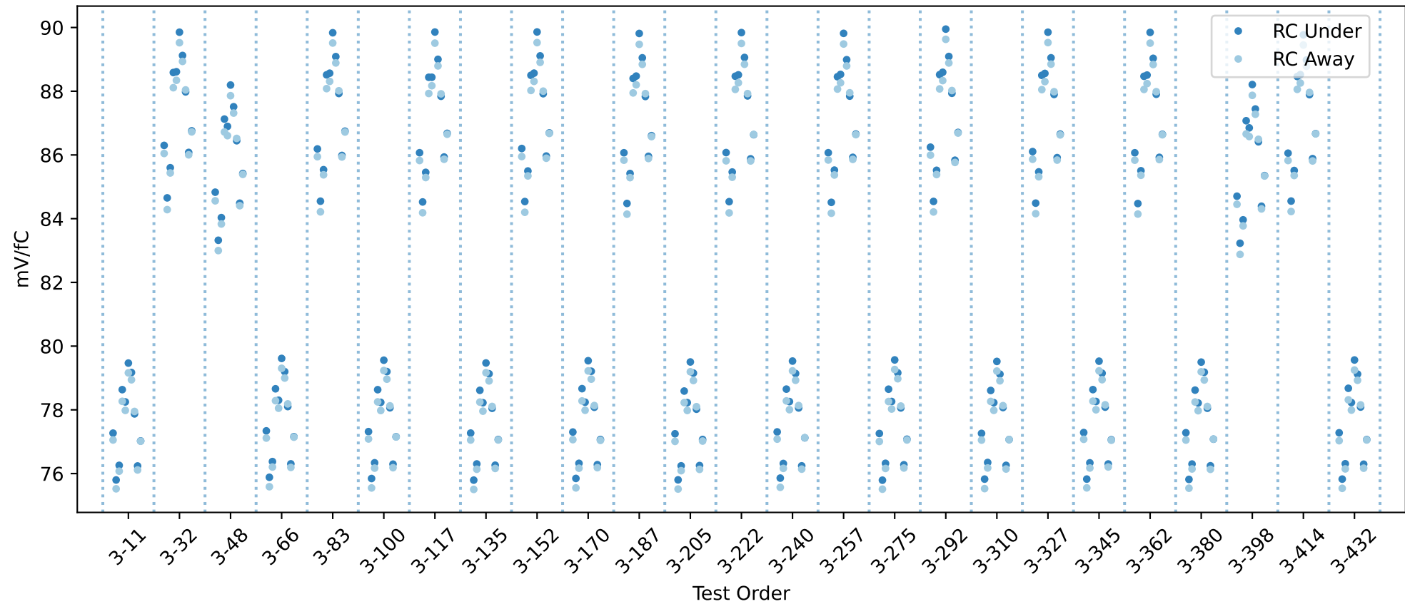
20USBHX2005235 RC gain chip averages
